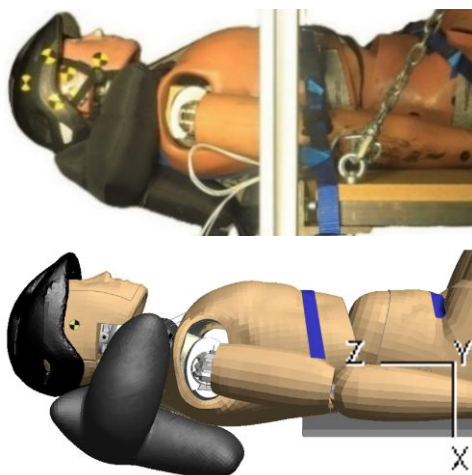
Fig. 1. H3 initial position in experimental testing (top) and in FE environment (bottom)
