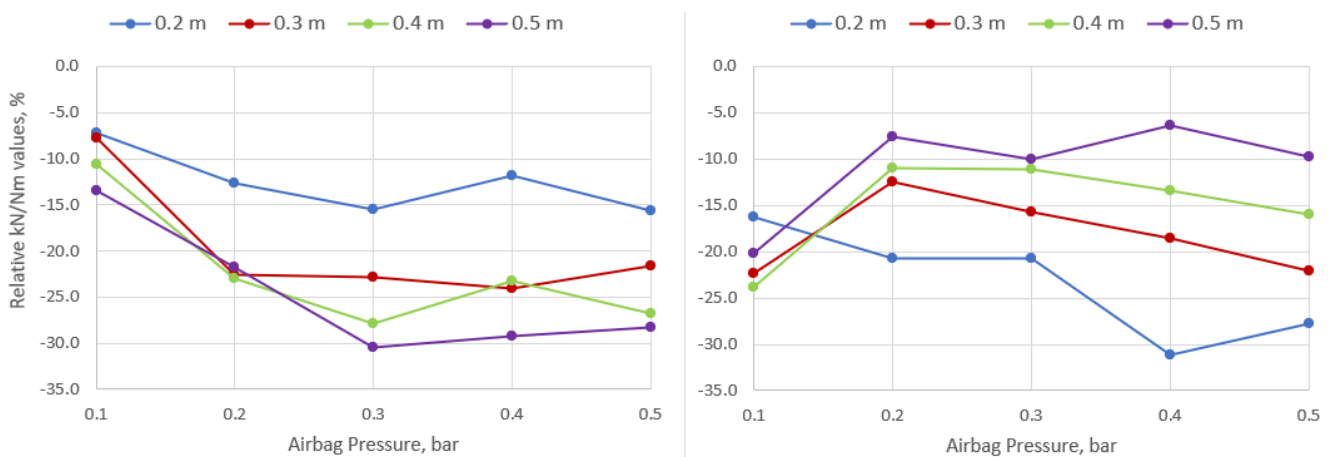
Fig. 8. PTW upper neck FY kN (left) and MX Nm (right) values, relative to the “no airbag” scenarios in all impact heights
