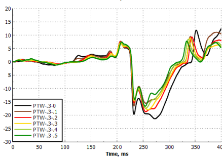
Fig. A9. Simulation responses for neck lateral flexion configurations of 20 cm (left) and 30 cm (right) fall heights
