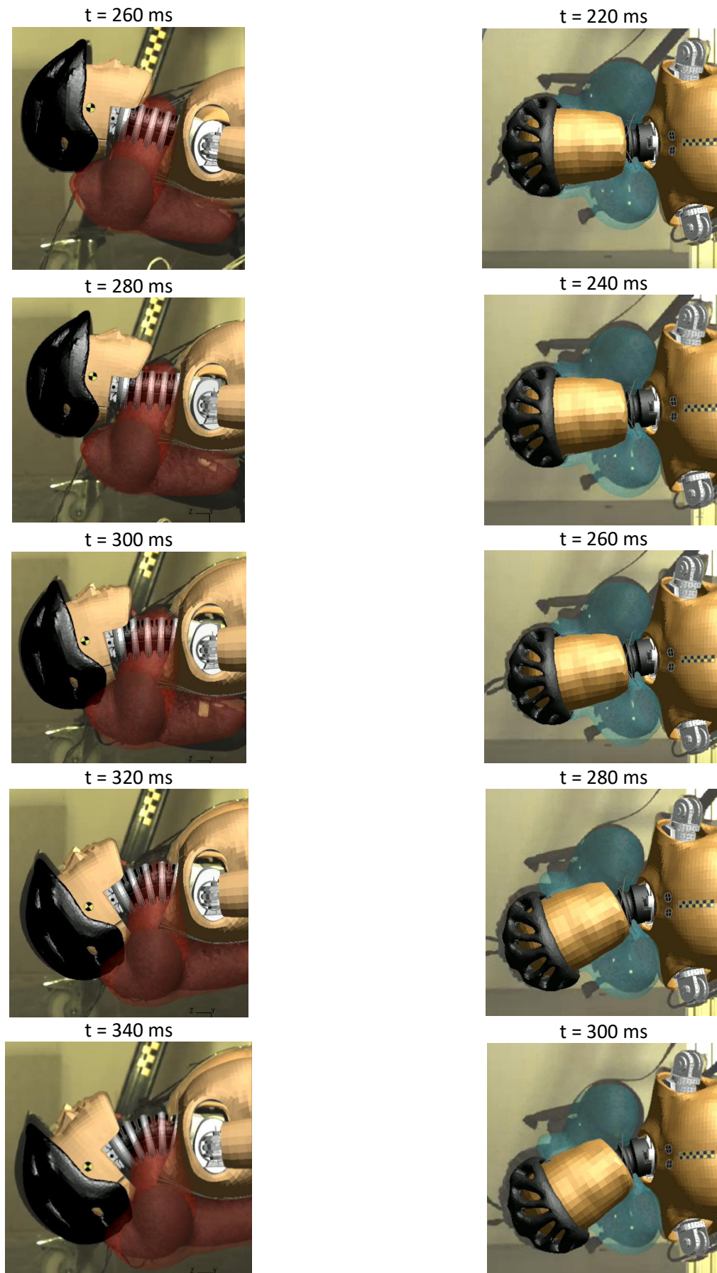
Fig. A2. Simulation versus experiment animation stills from impact initiation to maximum neck extension (left) and flexion (right): Airbag FE model boundary conditions validation based on kinematic behavior agreement between experimental and virtual testing
