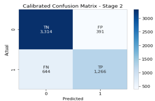
Figure 2: Confusion Matrix
