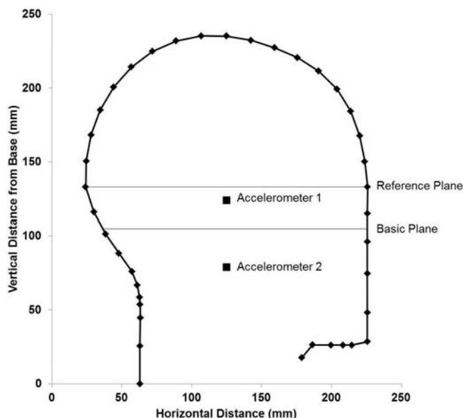
Fig. 2. Lateral cross section of the headform with Reference plane, Basic plane and accelerometer positions indicated.
