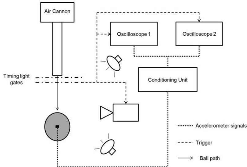
Fig. 3. Schematic of the equipment arrangement.
