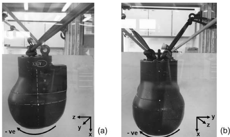
Fig. 1. (a) the headform orientation allowing frontal impacts (b) the headform orientation allowing lateral impacts. The ball was projected from right to left, parallel to the Z and Y axes respectively.
