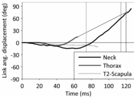
Fig. 4. Link angular displacements, test FSR02. Thorax angle was estimated from 65 ms to head impact.
