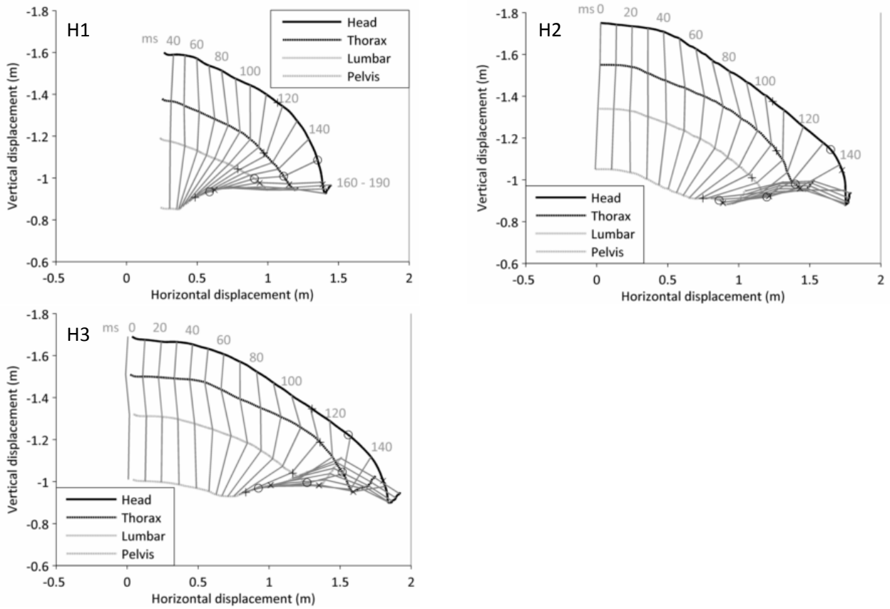
Fig. B1. Displacement relative to vehicle in test H1 (30 km/h), H2 and H3 (40 km/h). “+”, “o” and “x” mark elbow, shoulder and head impact time, respectively.
